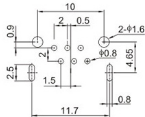
Recommend PCB Layout Jack Top View
