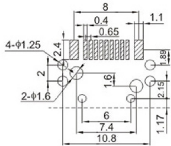
Recommend PCB Layout Jack Top View
